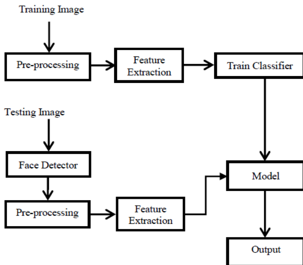
Fig 1: General approach for gender identification system
