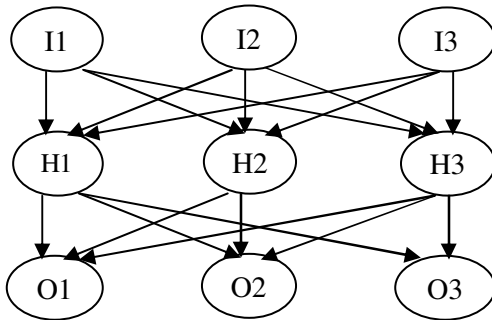
Fig 4. The structure of a back propagation network
