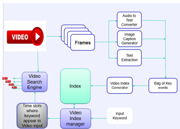
Fig 1 Video search using video index- Work flow
